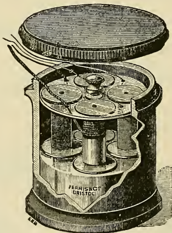
FIG. 226. — Author's reel holder; \frac{1}{2} size.
